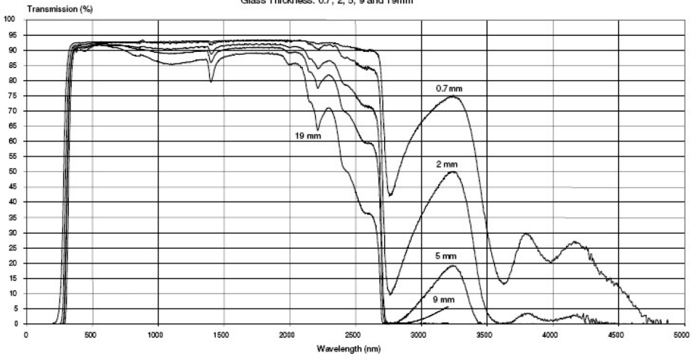
BOROFLOAT® Transmission Curve Glass Thickness: 0.7, 2, 5, 9 and 19mm
